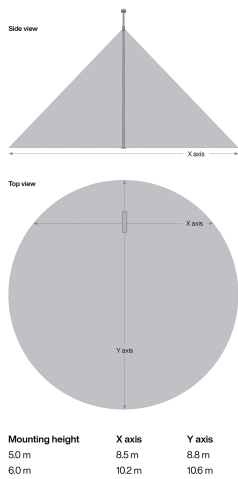
Detection zone "Mast Box Motion Low" 5EA3BGL01
